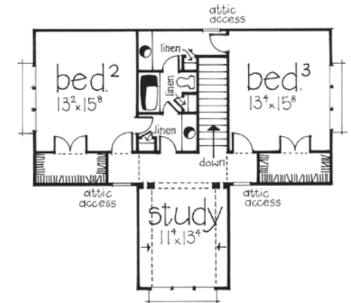
Floor 2
